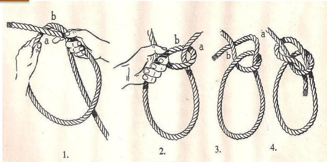
Figura 1.10 As de guía
